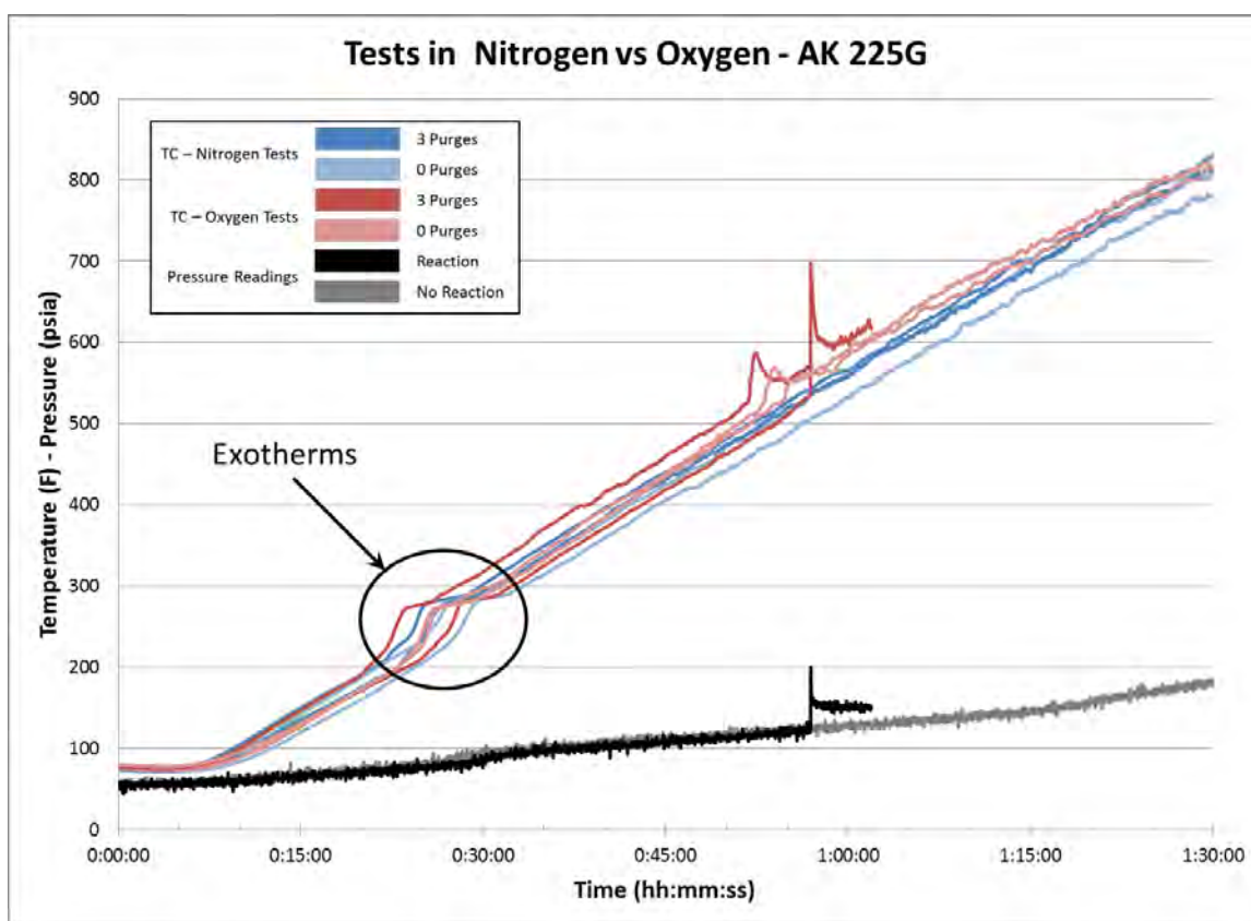
Figure 8 Exotherm Evaluation
