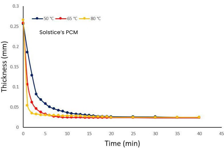
Figure 3. BLT changes as a function of heating time. Samples subjected to three temperatures.
