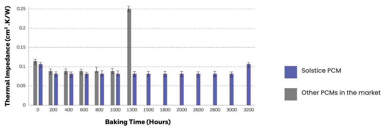
Figure 4. Comparison between typical PCM and Solstice PCM for AI applications: high temperature baked at 150C over 3,000 hours. Thermal impedance (TI) properties comparison between typical PCM and Solstice PCM for the AI industry. Test method: Laser Flash, ASTM E1461. Solstice PCM delivers TI of less than 0.1 cm².K/W and high thermal stability over time, providing excellent long-term wetting and reliability. TI of PCM slightly decreases after 200 hours due to improved wetting and remains stable thereafter.
