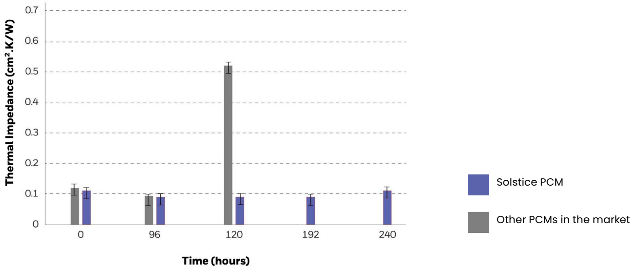
Figure 5. TI performance of PCM undergoing a highly accelerated stress test.
