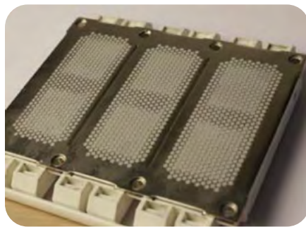
PTM6000HV-SP applied to IGBT module
