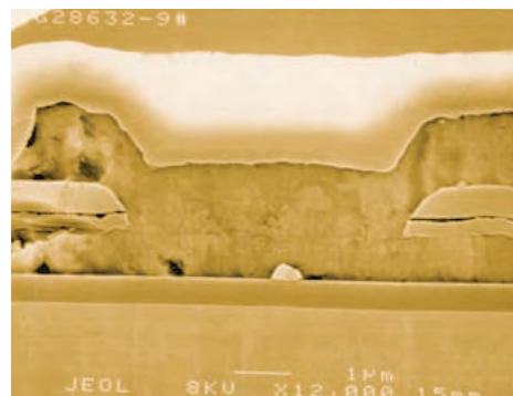
CVD/P-112LS/CVD sandwich structure. (SEM courtesy of ASMC)
