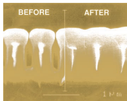
T-14 fills reentrant gaps as small as 0.1µm created by non-conformal CVD \text{SiO}_2 deposition.
