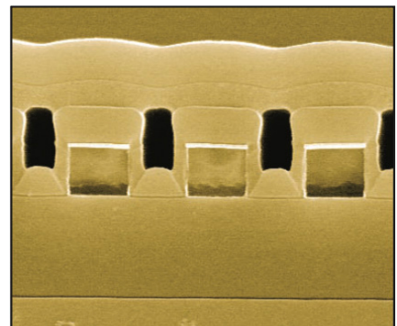
ACCUGLASS T-11 planarizes and fills gaps to 0.35µm.
