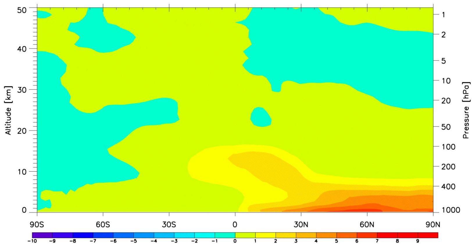
Figure 4. Change (%) in annual, zonal mean \text{Cl}_y mixing ratio derived for Perturbation 1, the scenario in which currently used blowing agents have been substituted by tCFP and the used tCFP is completely released to the atmosphere, relative to the reference scenario.
