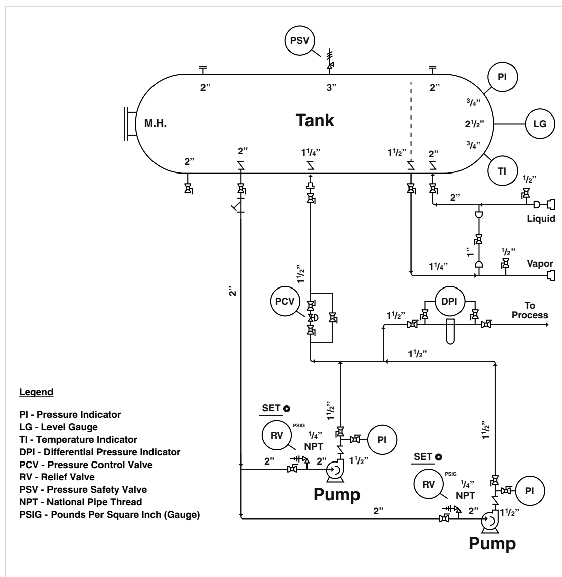
Drawing 2
