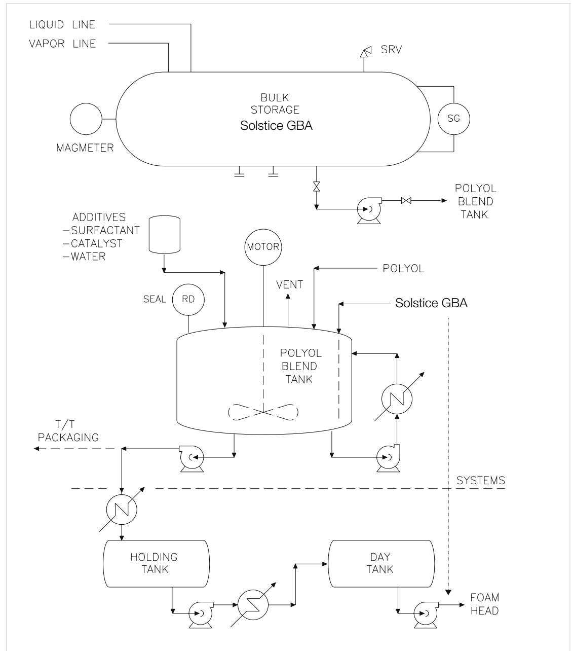
Drawing 6
